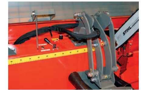
The AC 10 automatic chain tensioner maintains optimal saw chain tension at all times. The chain can be conveniently replaced after releasing chain tension with the lever pictured – no tools required!
