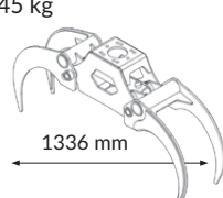
Branch grapple 0.24 145 kg
