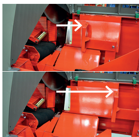
Adjustable splitting length from 250 mm up to 550 mm.
